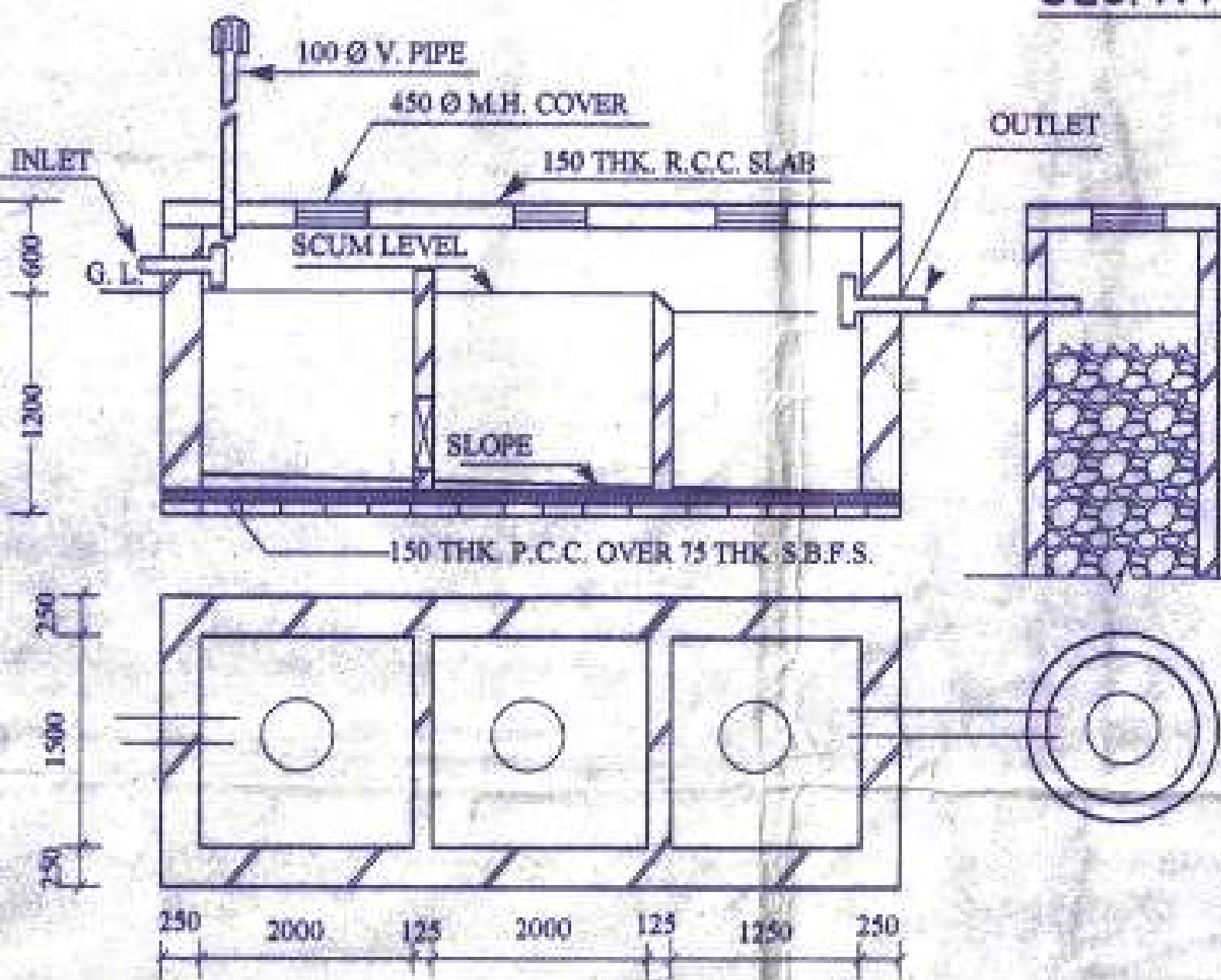
DETL. OF SEPTICTANK & SOAK PIT (FOR 50 USER)
